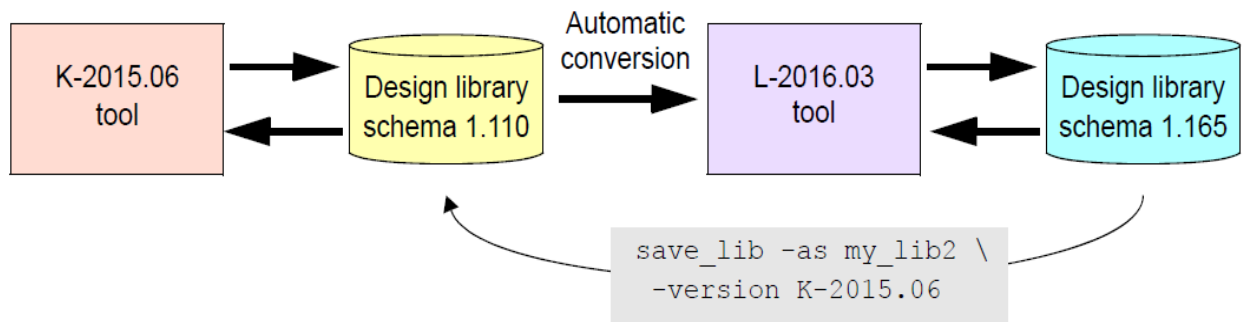
Figure 31 NDM Database Schema Compatibility
